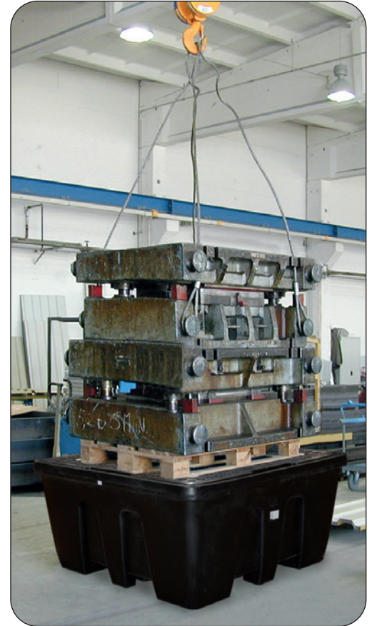
PE-KT-1S under a test load of 8.000 kg
